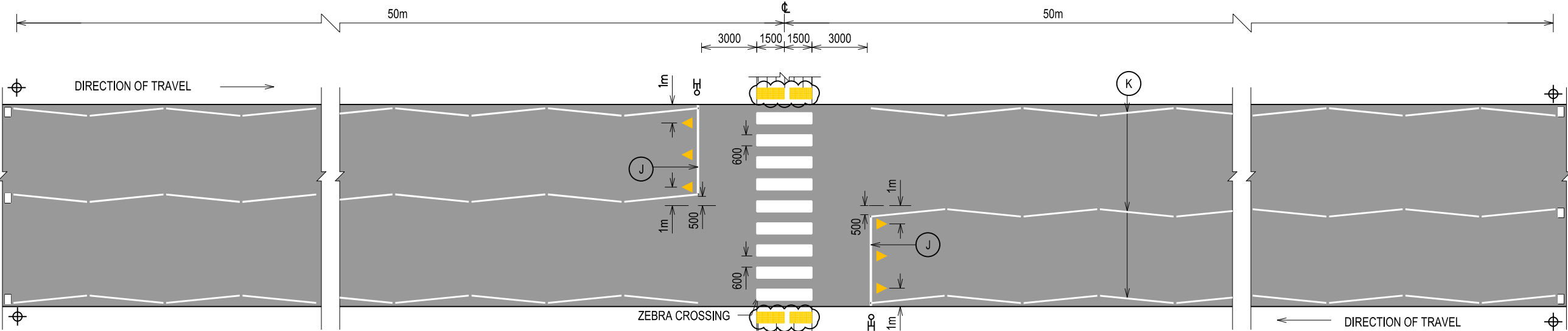
ZEBRA CROSSING AND ZIG ZAG MARKING
