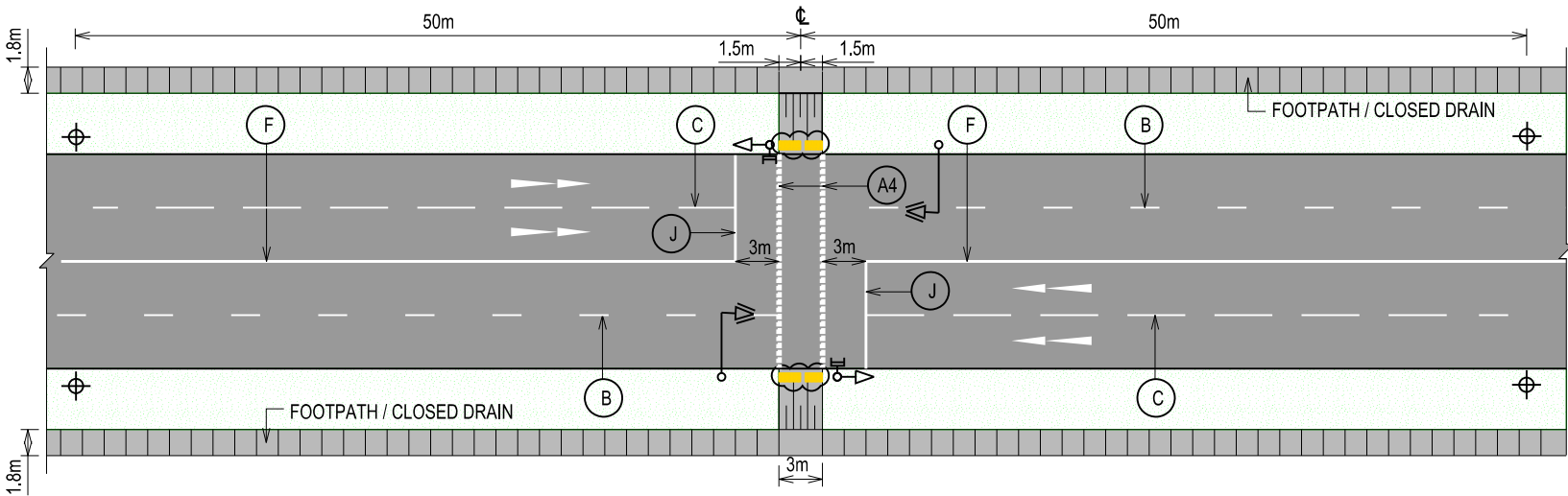
SIGNALISED PEDESTRIAN CROSSING
