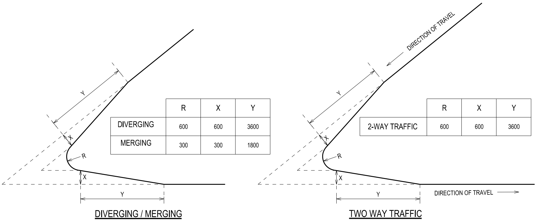
NOSING AT CHANNELISING ISLAND SCALE 1:100
