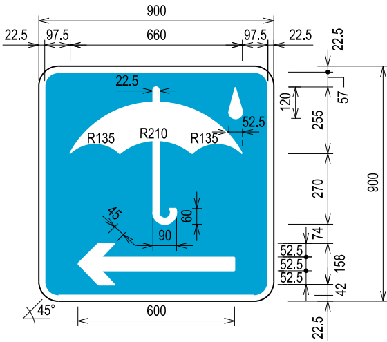
RAIN SHELTER SIGN
