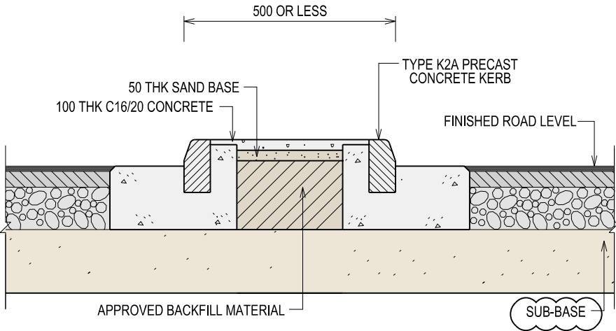
DETAILS OF PAVED SURFACE SCALE 1:25
