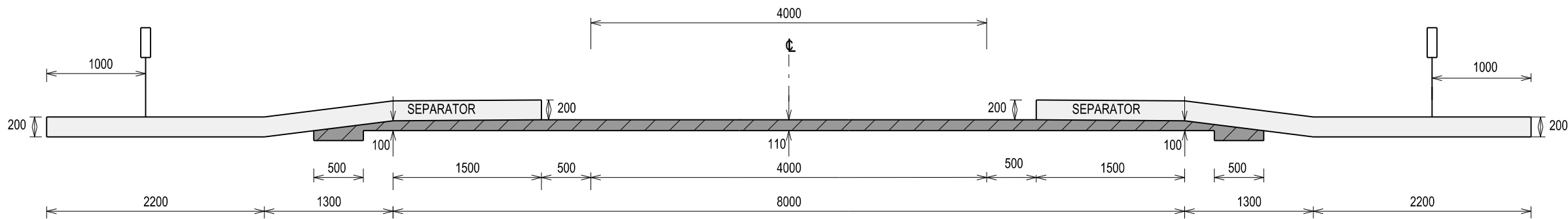
SECTION A-A SCALE 1:50
