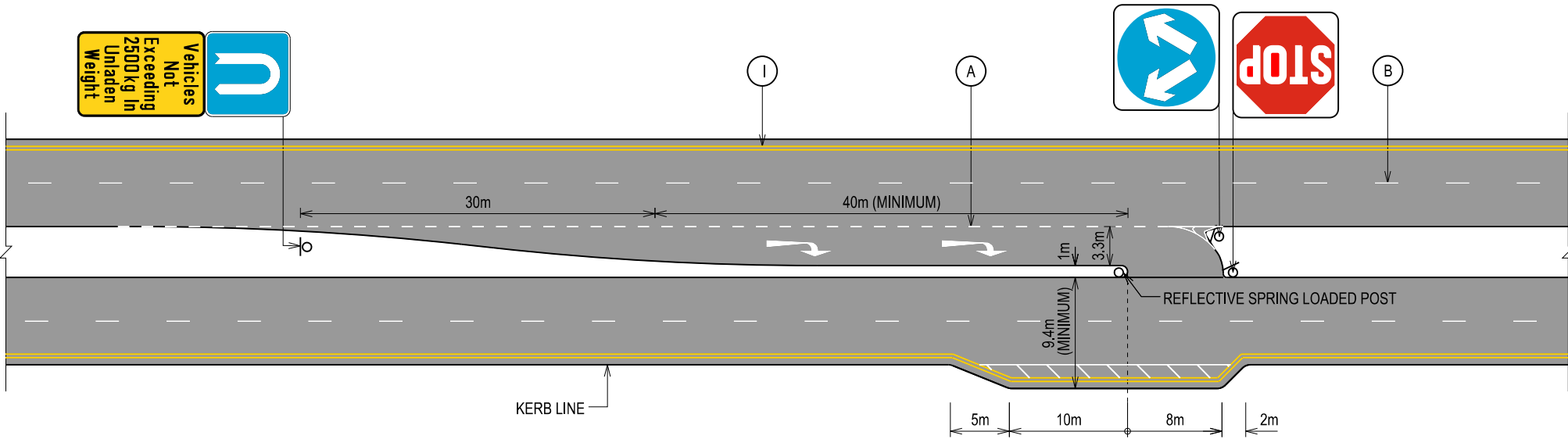
DETAIL OF U-TURN LESS THAN 2500kg (2 LANES CARRIAGEWAY) SCALE 1:500
